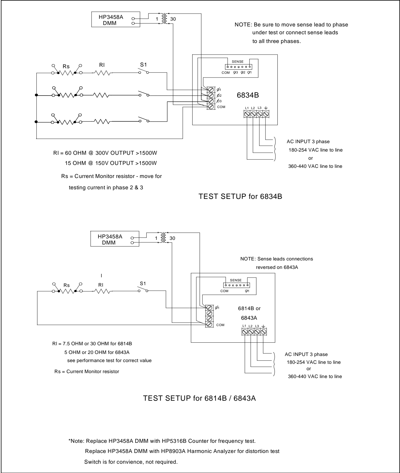
Figure 2-1. Verification Test Setup
