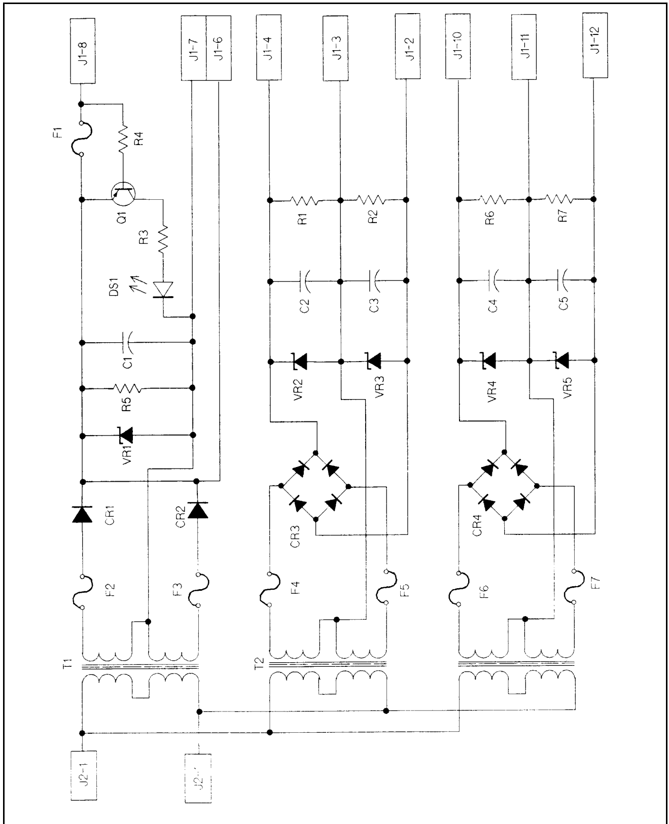
Figure 6-10. A14 Bias Power Supply Assembly Schematic
