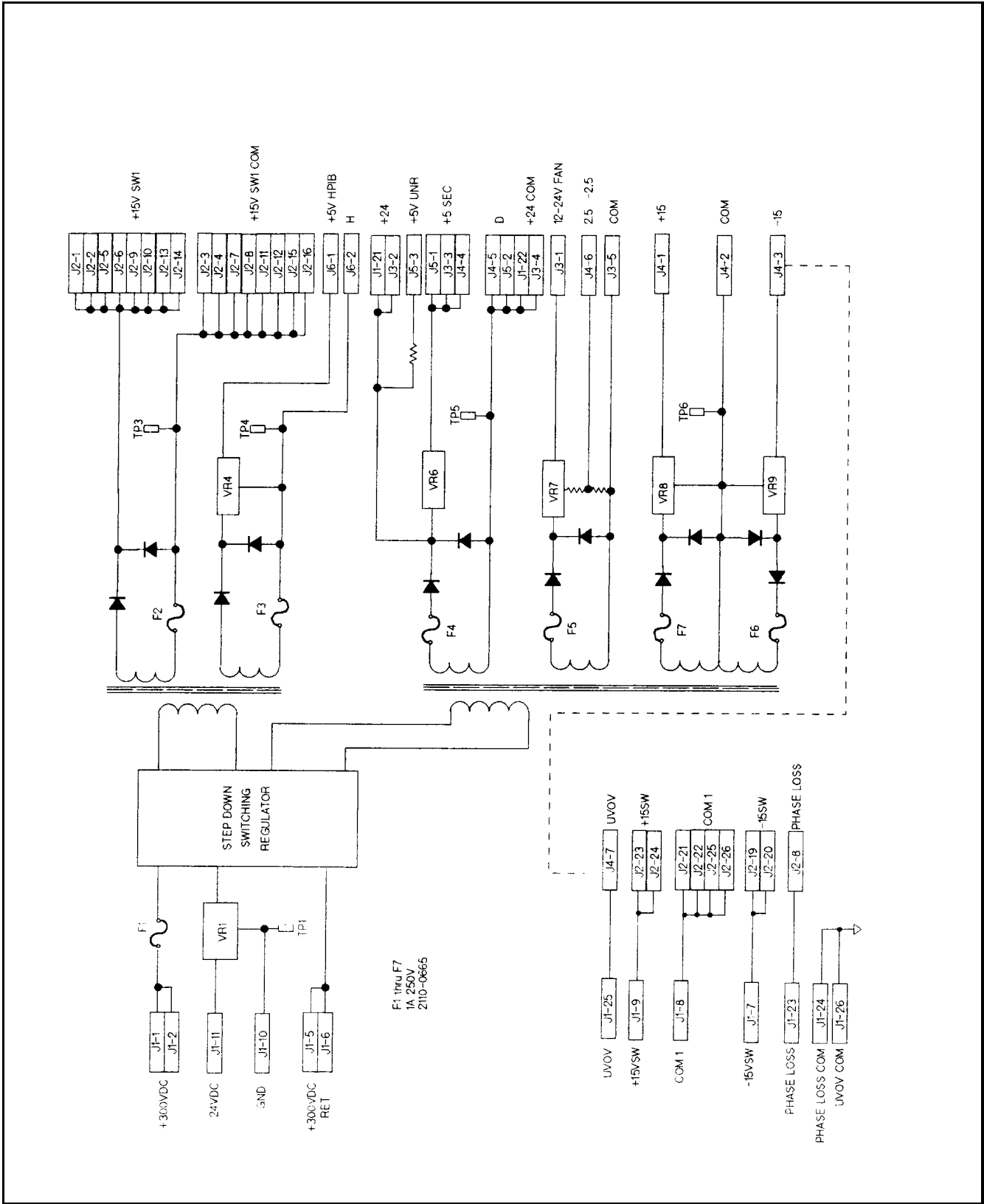
Figure 6-8. A10 Auxiliary Power Supply Assembly Schematic
