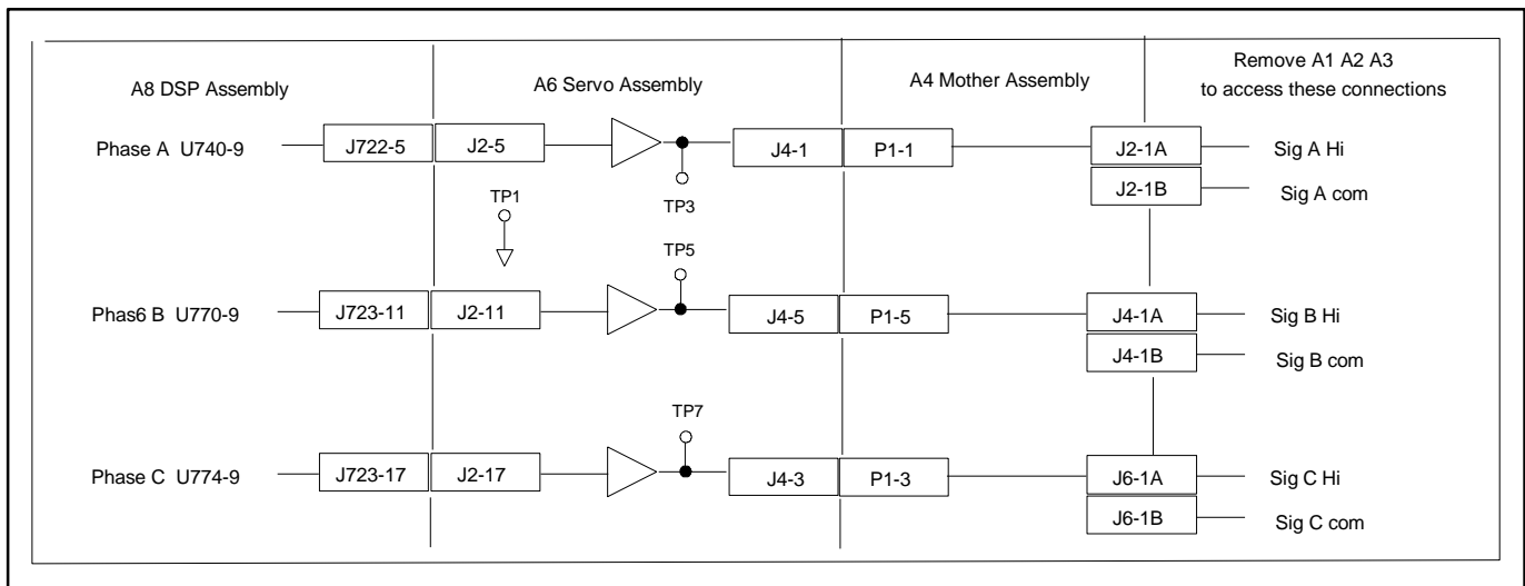
Figure 3-2. AC Programming Signal Path
