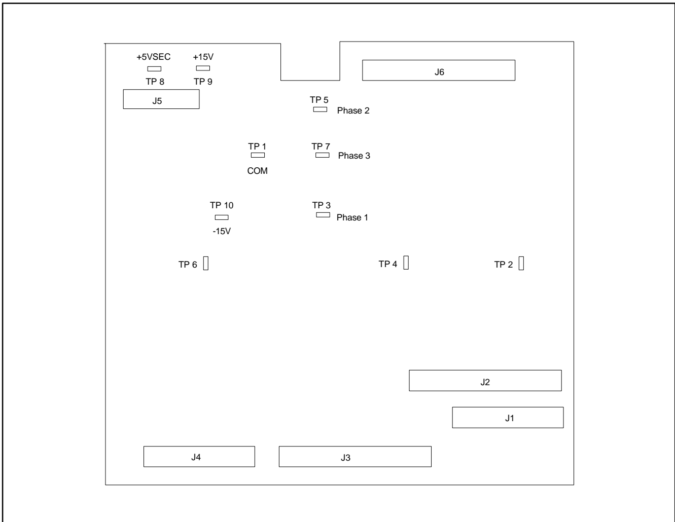
Figure 6-15 A6 Servo Board Test Point Location
