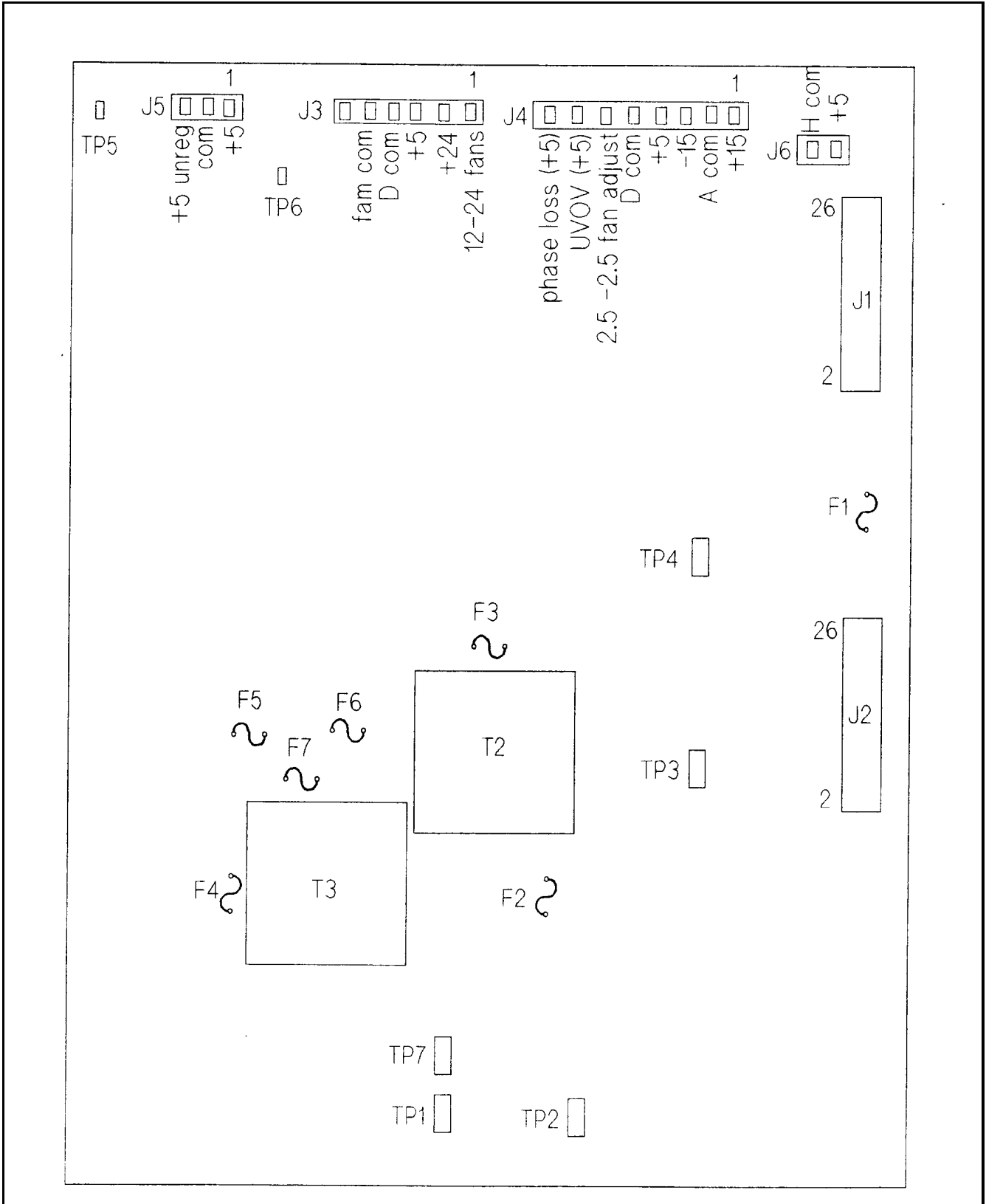
Figure 6-7. A10 Auxiliary Power Supply Board Parts Location
