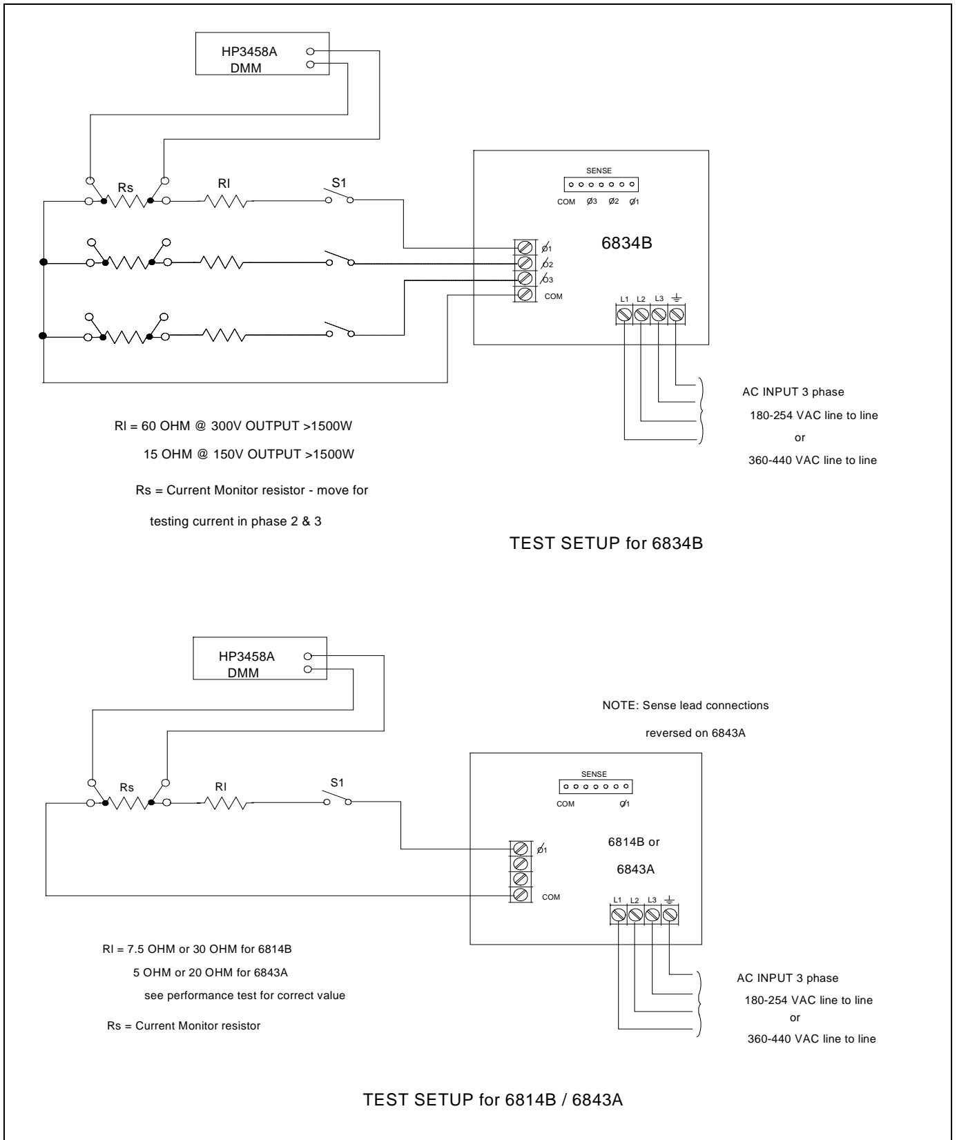
Figure 2-2 Verification Test Setup
